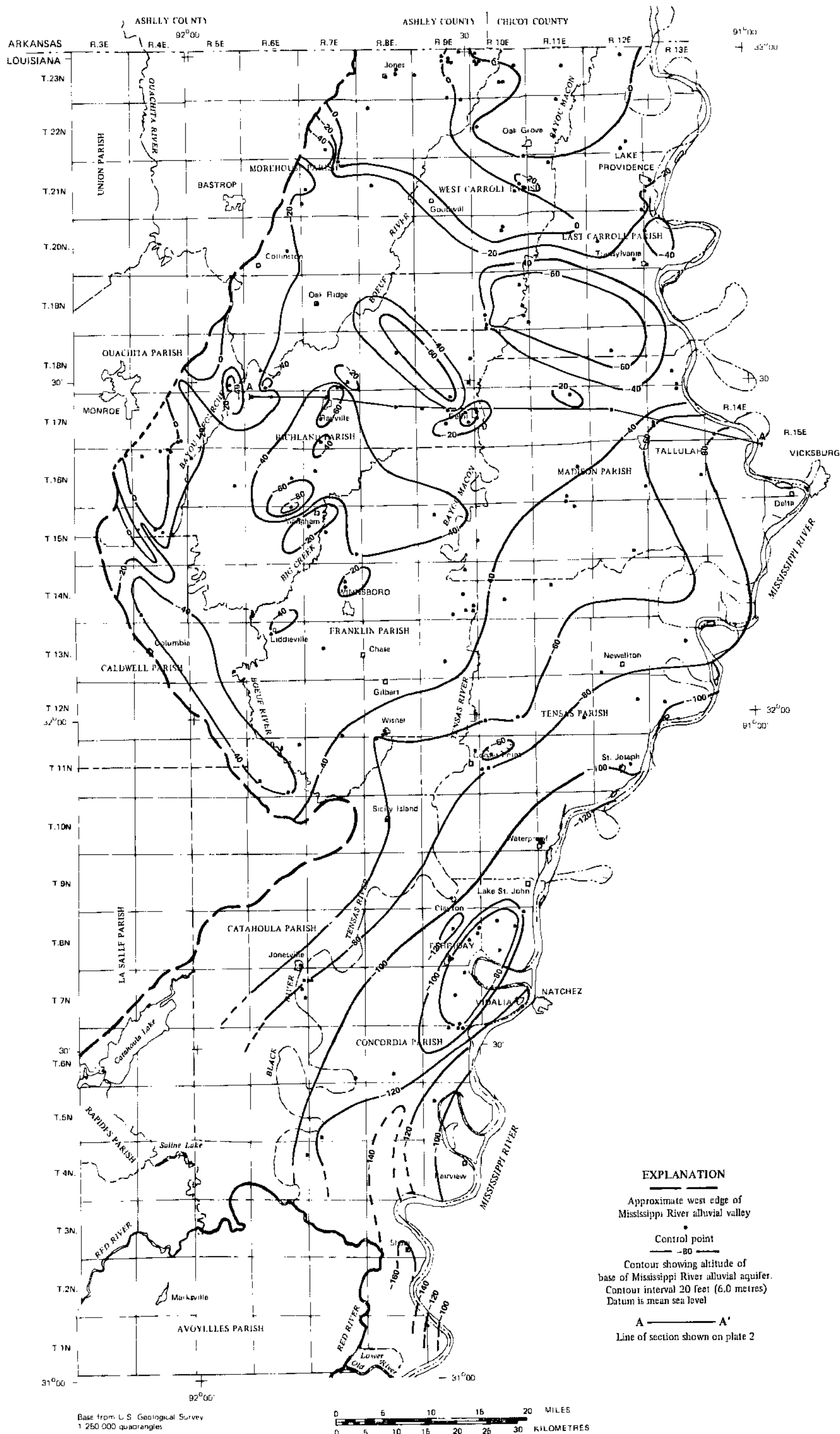
PLATE 3. MAP SHOWING ALTITUDE OF BASE OF THE MISSISSIPPI RIVER ALLUVIAL AQUIFER, LOUISIANA.
