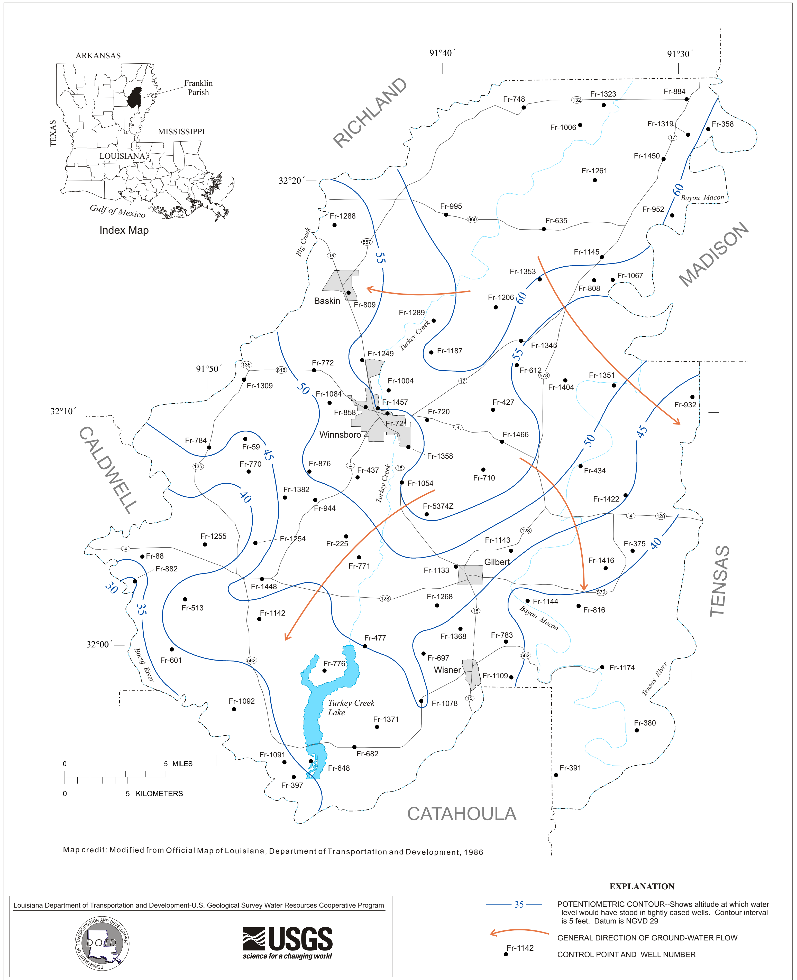
Plate 1. Potentiometric surface of the Mississippi River alluvial aquifer, Franklin Parish, Louisiana, October 2001.
