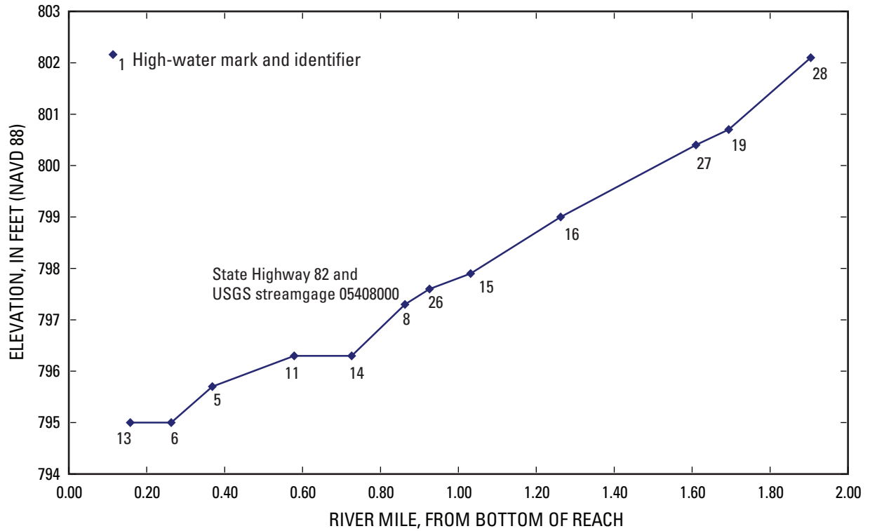
Appendix 3D. Flood-peak water-surface profile with selected high-water marks for the Kickapoo River at La Farge, Wisconsin, for flood of June 2008. Elevation is referenced to North American Vertical Datum of 1988 (NAVD 88).
